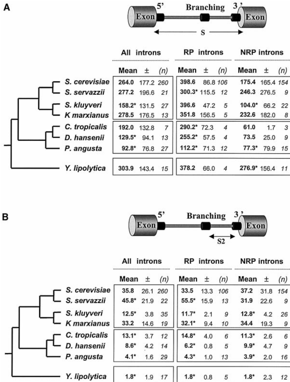
Figure 3. Yeast spliceosomal intron length. (A) Phylogenetic evolution of mean intron size in all introns, and in genes encoding NRPs and RPs. (B) Phylogenetic evolution of the mean S2 distance, e.g. the internal distance between the branch motif and the 3' splice motif in: all introns, in genes encoding NRPs and in those encoding RPs. For each yeast species and each intron population: the mean intron size (Mean), the standard deviation ( \pm ) in nucleotides and the number of introns analysed ( n ) are indicated. Panels illustrate the main phylogenetic subdivisions. The asterisk represents that this value was found to be statistically different from that observed in S.cerevisiae at P = 0.05 .
