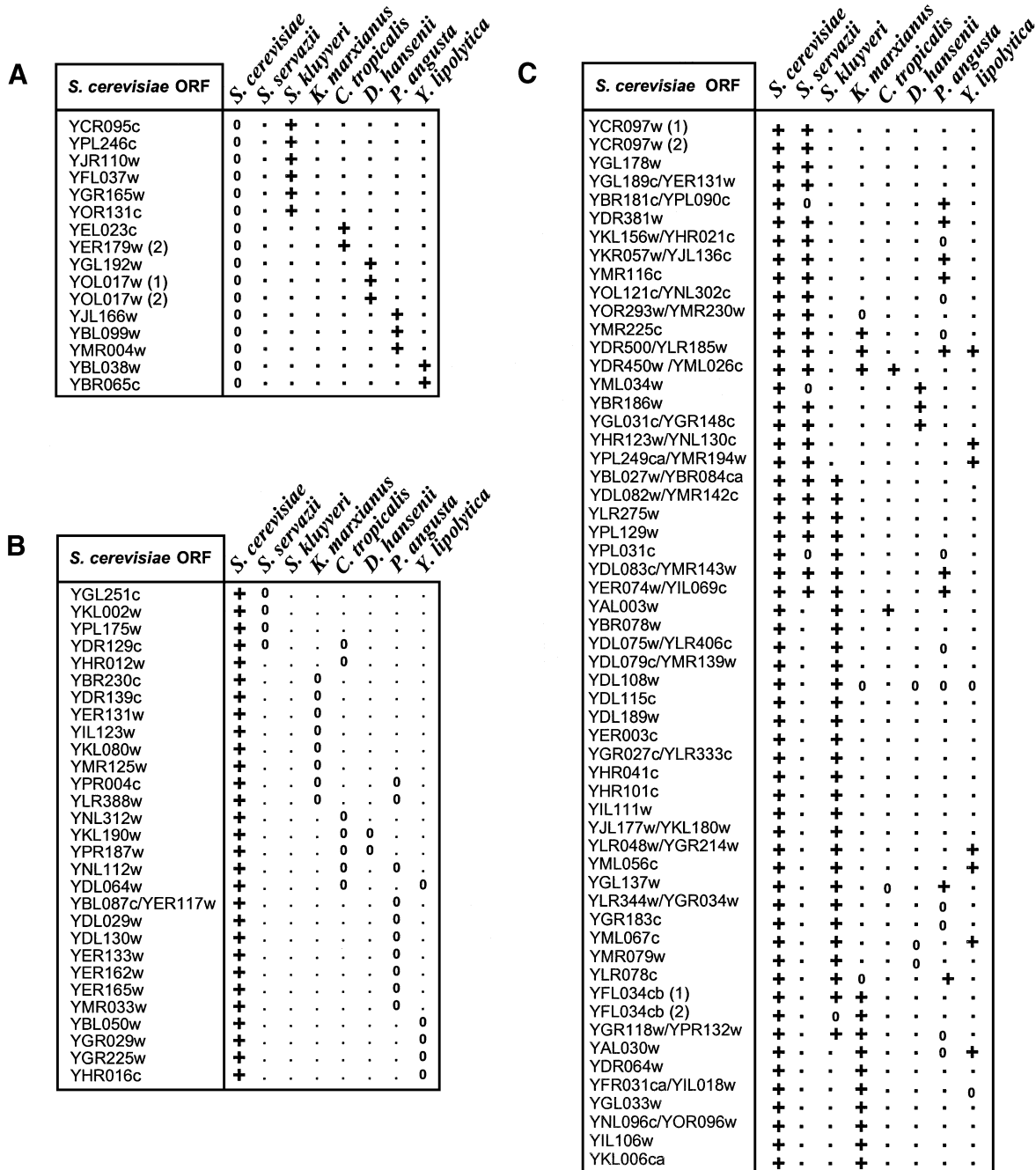
Figure 4. Presence or absence of introns in homologous genes of hemiascomycetous yeasts. A group of 52 introns was shown to be present in at least three yeast species. This figure indicates whether each intron was present or absent in each yeast species. The name of the S.cerevisiae ORF is indicated on the left. The presence of an intron is indicated by '+' and its absence by '0'. The symbol '.' indicates that the homologous gene was not found in our DNA library. Introns apparently restricted to a yeast species other than S.cerevisiae are in (A), those restricted to the S.cerevisiae species are in (B), and those that can be considered to be 'ubiquitous' are in (C).
