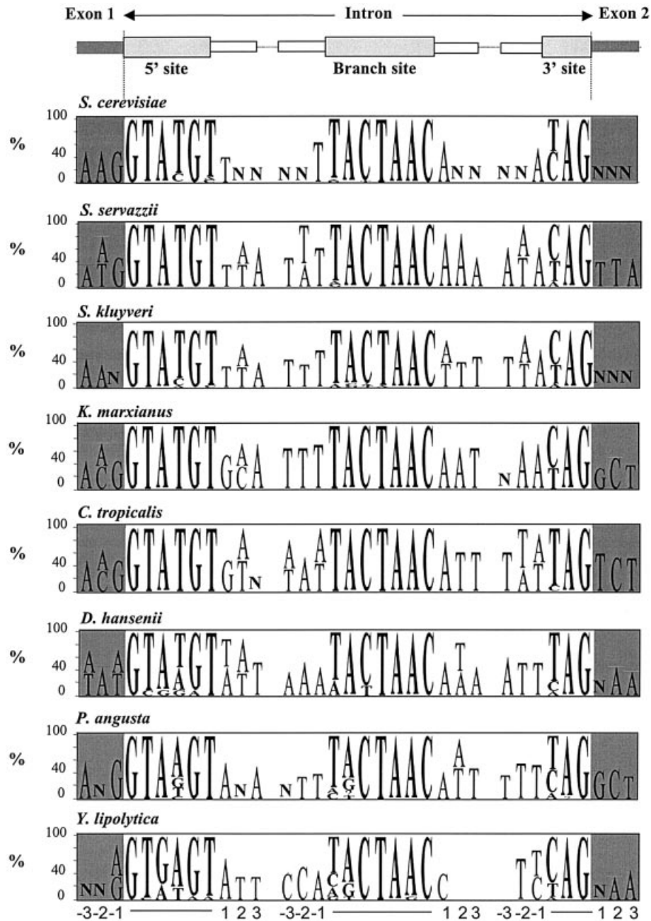
Figure 2. Preferential nucleotide usage around splicing sites. The vertical and horizontal axes represent the frequencies and positions of nucleotides, respectively. The height (expressed as a percentage) of each letter is proportional to the frequency of each base at each position.
