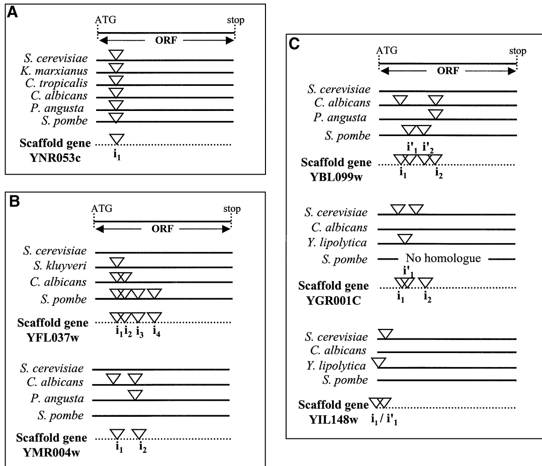
Figure 5. Conservation of intron positions. Examples of the tracking of intron positions between homologous yeast genes. (A) Conserved intron positions. (B) Missing intron positions at the 3' end (YFL037w) or at the 5' end (YMR004w) of the gene sequences. (C) Divergent intron positions in poorly (YBL099w) or highly (YGR001c, YIL148w) conserved regions. The horizontal lines illustrate the different sequences aligned by ClustalX. Intron positions are indicated by the inverted triangle symbol. A scaffold gene is indicated by dashed lines in each example.
